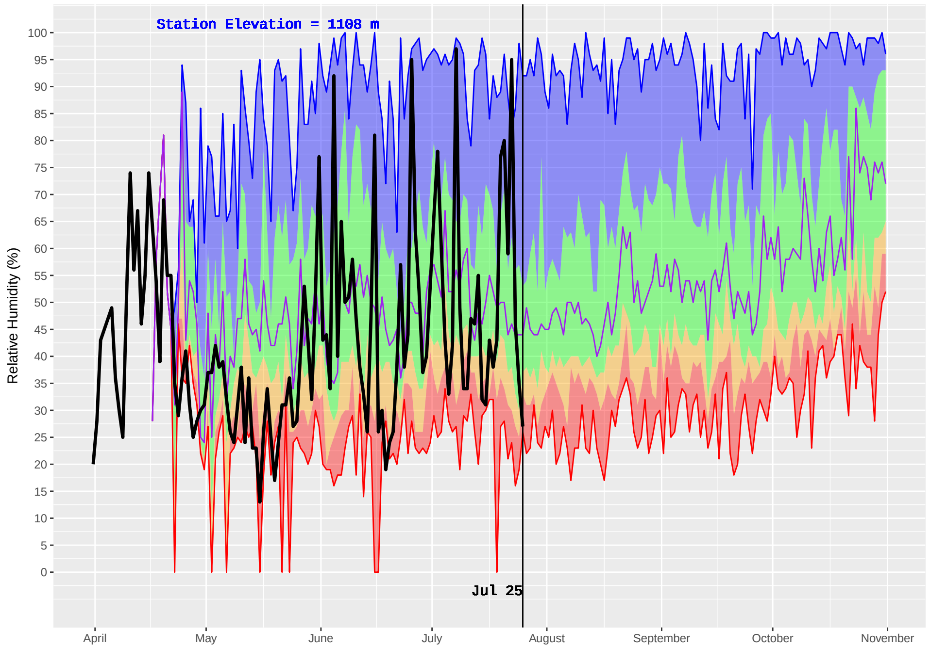
NABESHE (151) : Historical (1987–2016) and Current (2018) Noon Relative Humidity
