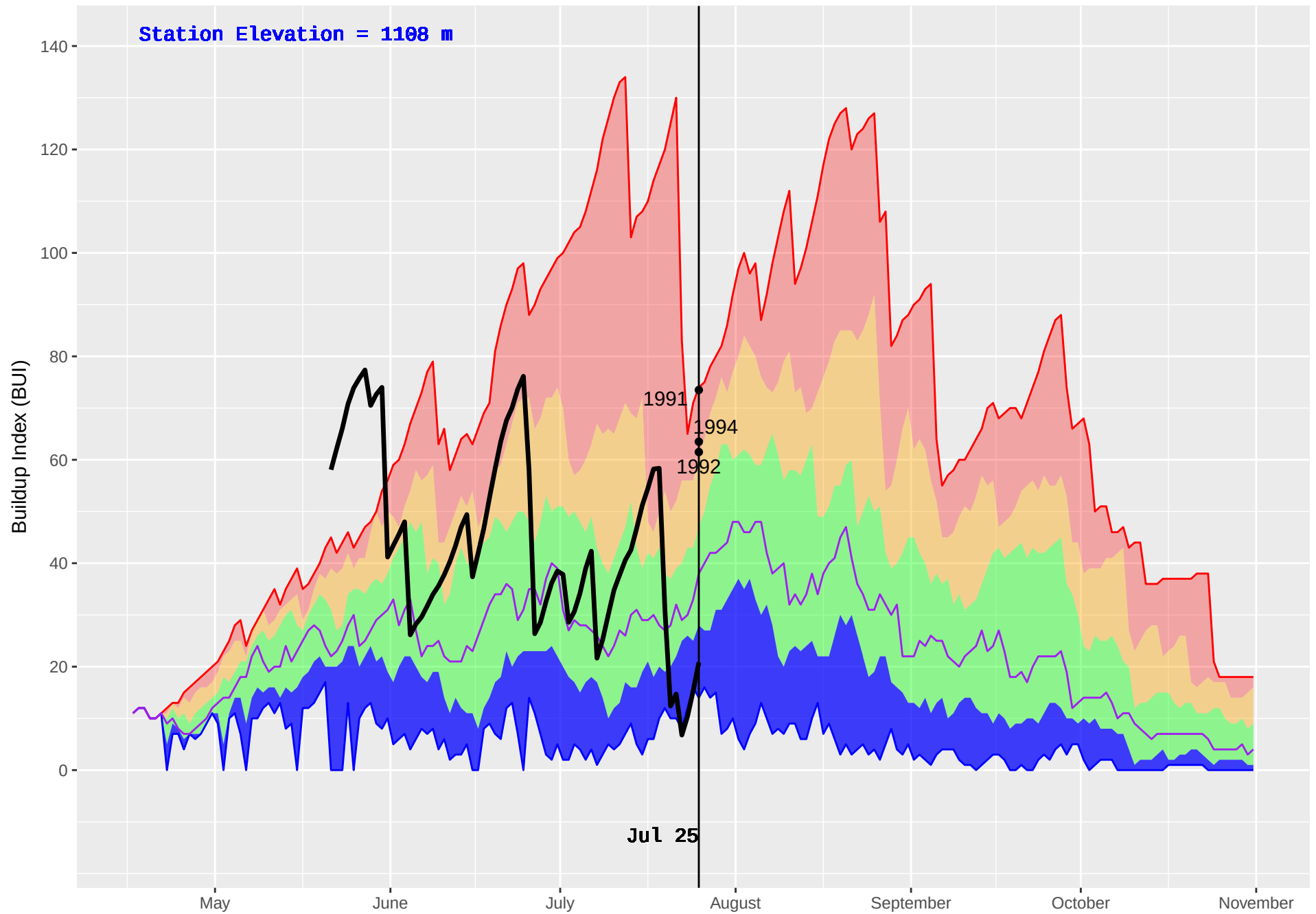
NABESHE (151) : Historical (1987–2016) and Current (2018) Noon Buildup Index (BUI)
